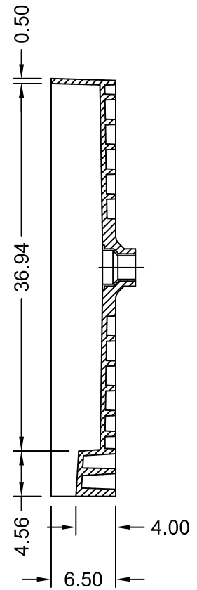
SECTION B-B
